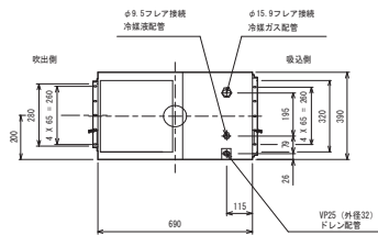
P71LFU12.DXF
