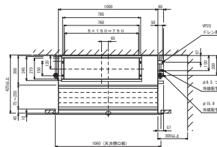
P71T1112.DXF
