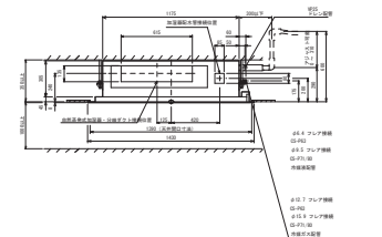
P71L1U12.DXF
