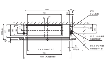
P71FFU12.DXF
