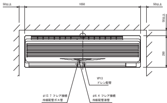
P71D1U12.DXF
