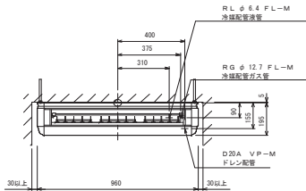
P63DG112.DXF
