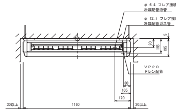
P71EFUN2.DXF
