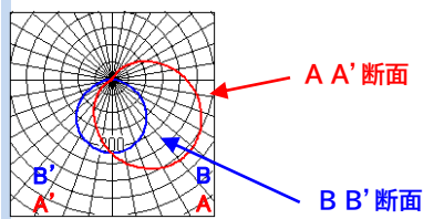
図2 配光曲線:XLX450CBLC
