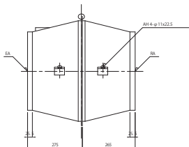
45MTV304.DXF
