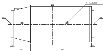
45DST004.DXF
