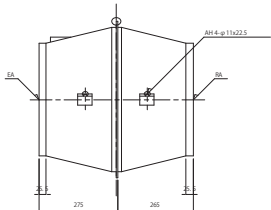
45DTL004.DXF
