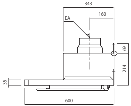
60DED2S4.DXF
