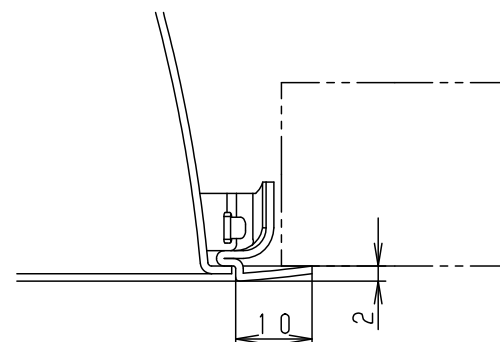
枠部詳細 (S = 1 / 1)
