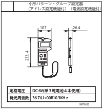
WRT9630.DXF
