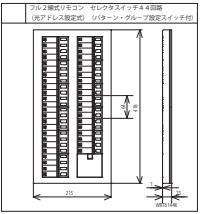
WRT9630.DXF
