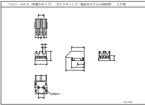
DH5857K.DXF
