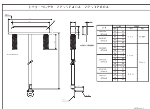
DH6111.DXF
