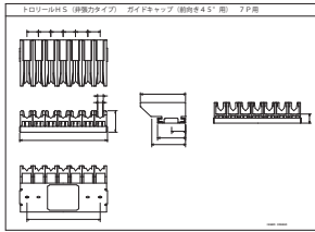
DH5855K.DXF
