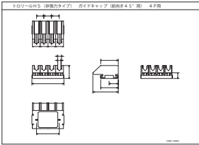
DH5862.DXF
